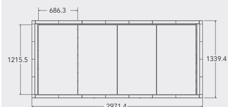
Wall-mount – Side view
