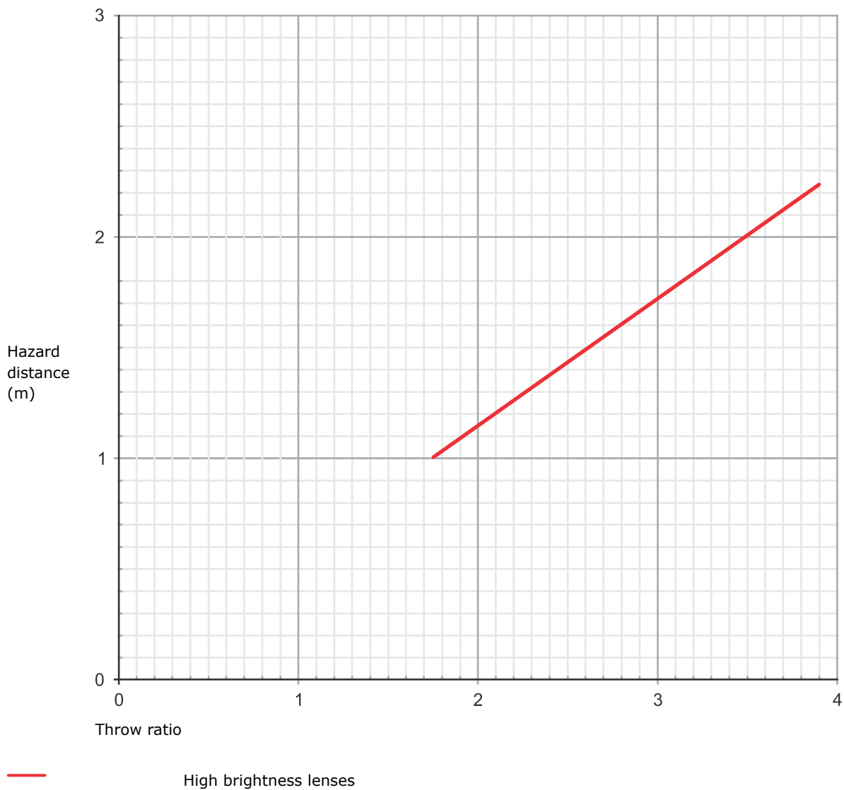
CP2411-RBe hazard distance table and graph
