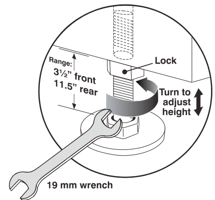
Figure 2-6 Adjust Feet
