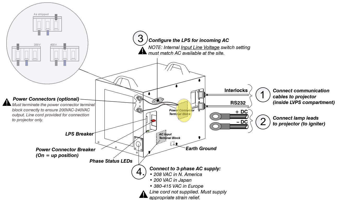
Figure 2-15 Connect LPS
