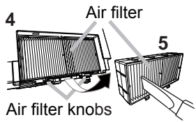
Filter vent
