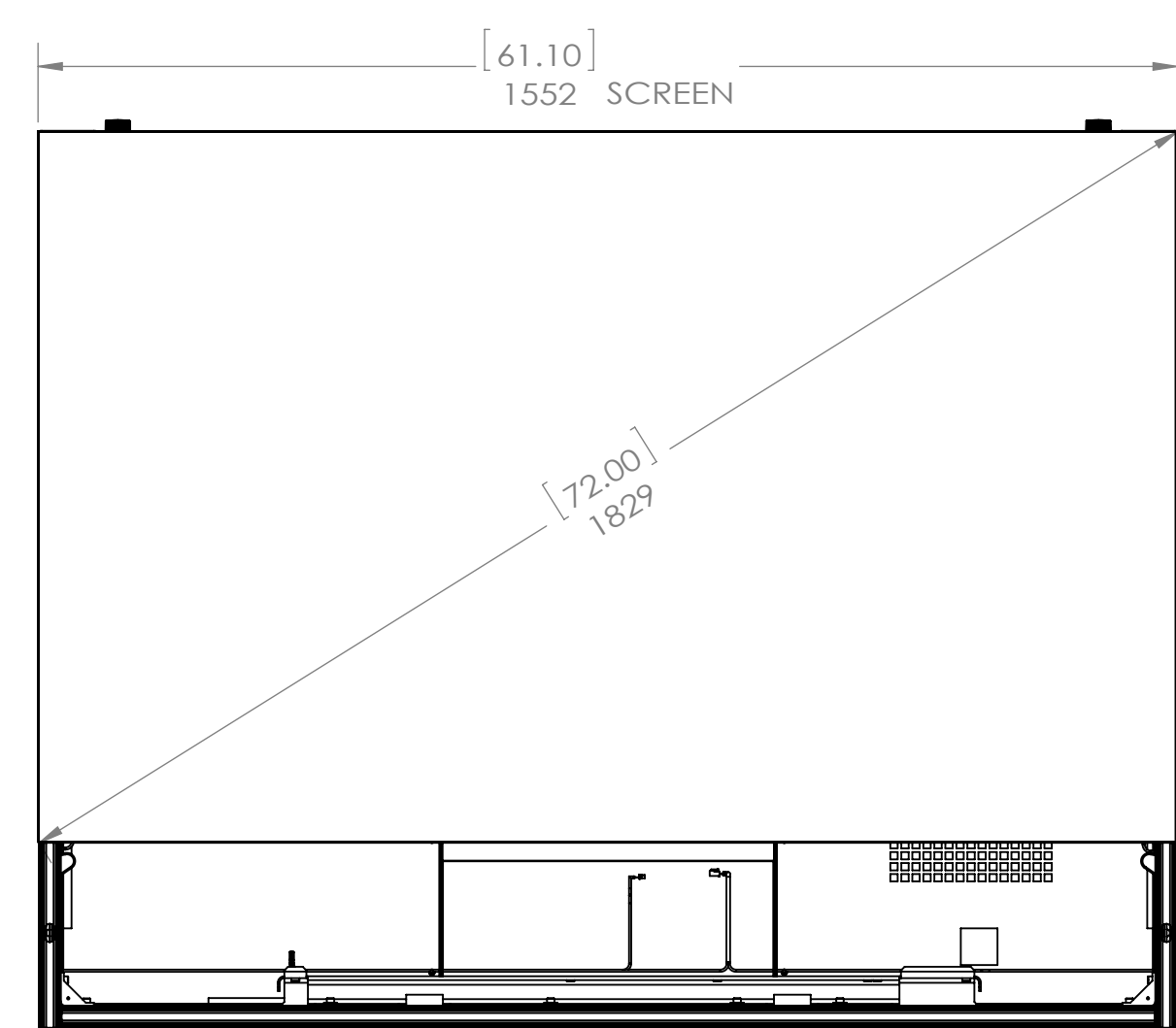
FRONT VIEW
