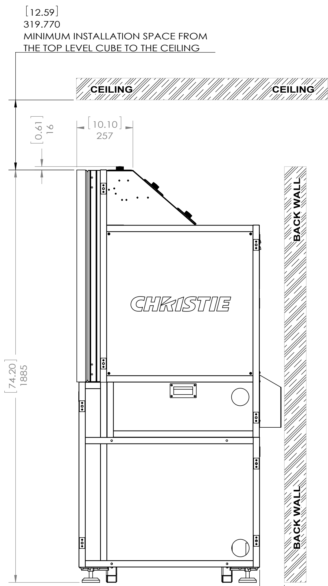
SIDE VIEW
