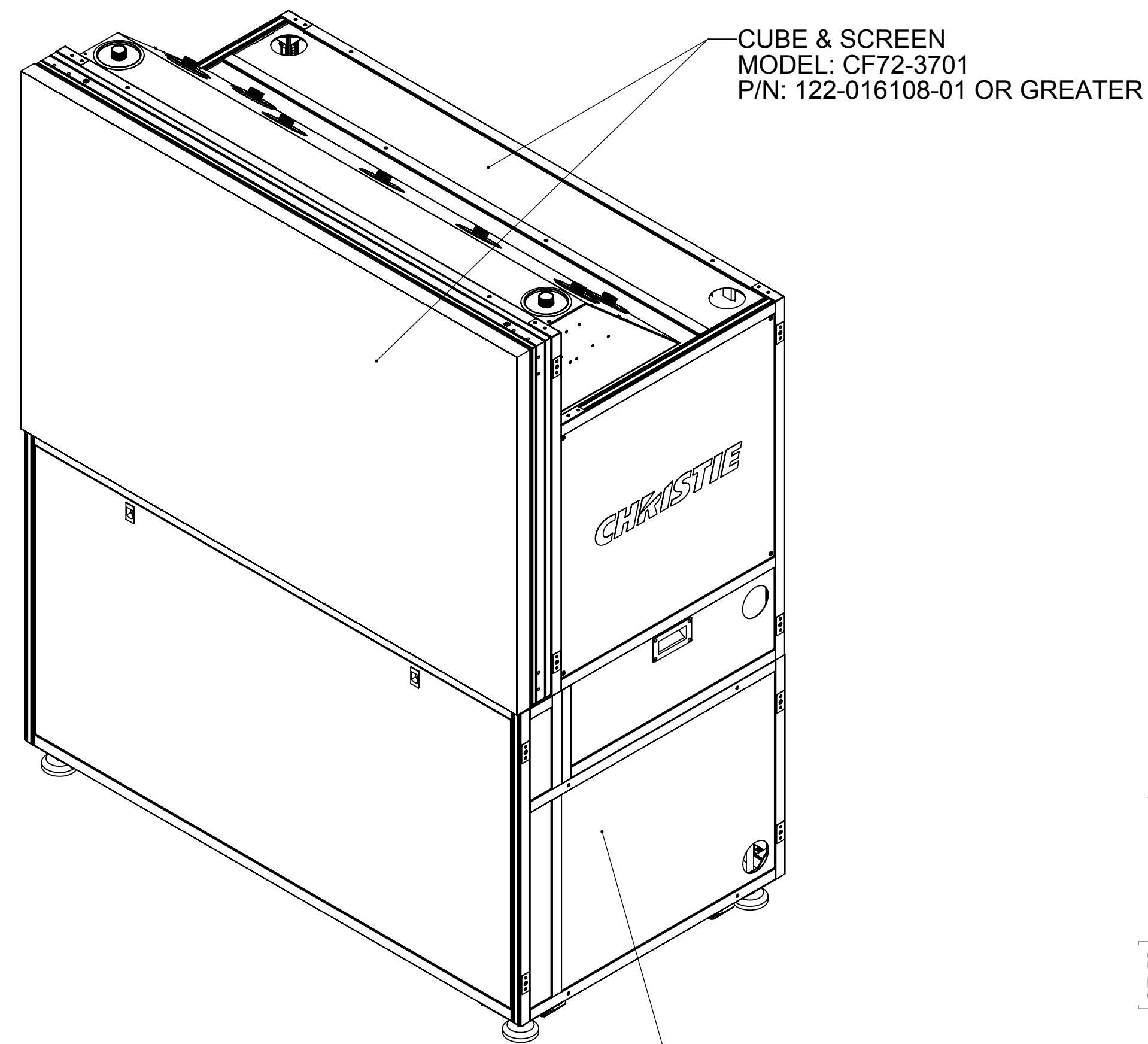
ISOMETRIC VIEW
