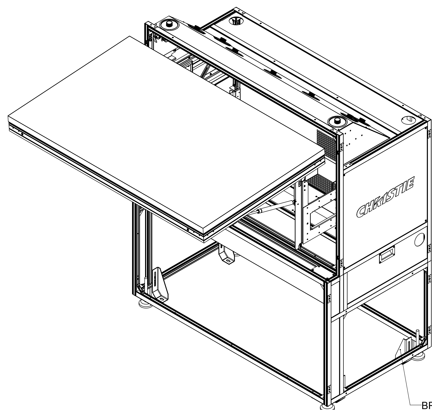
ISOMETRIC VIEW
