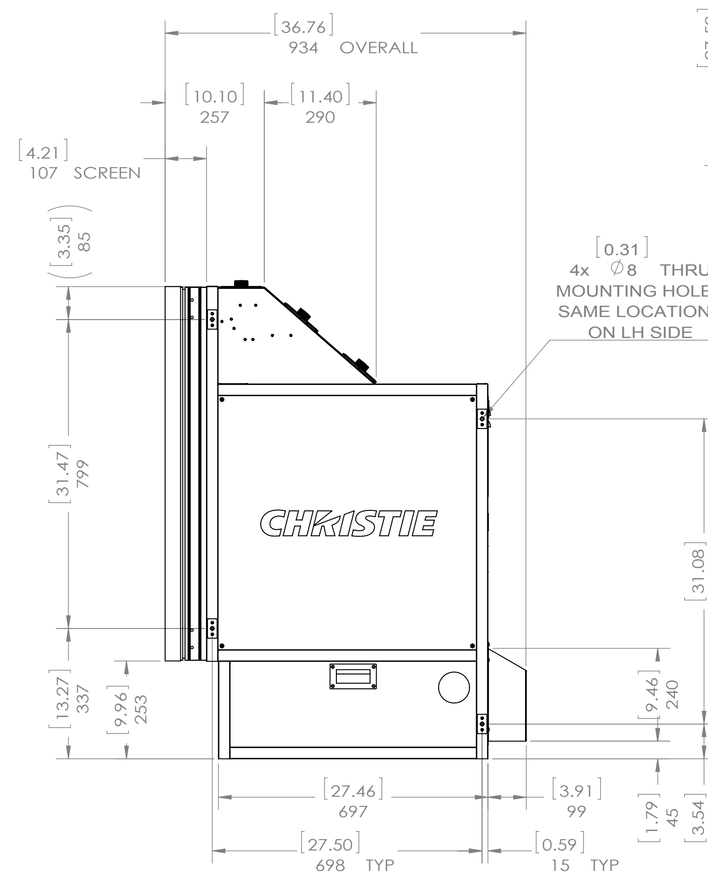
SIDE VIEW
