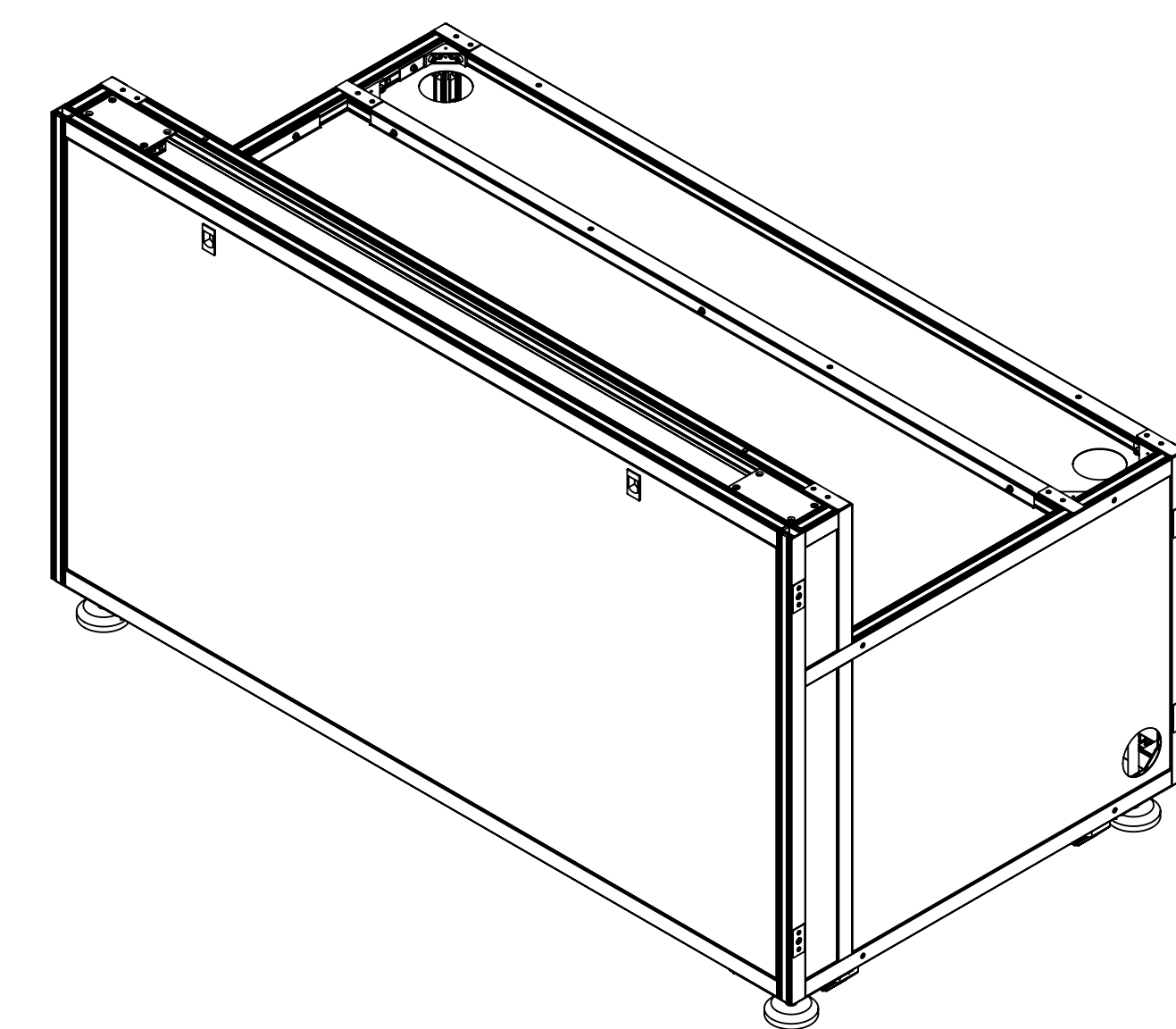
ISOMETRIC VIEW
