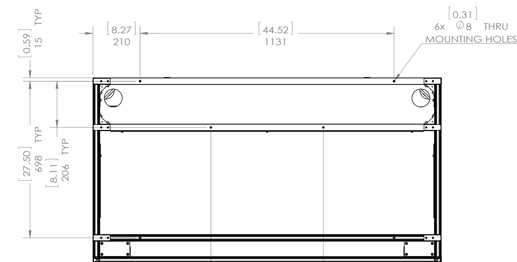
TOP VIEW
