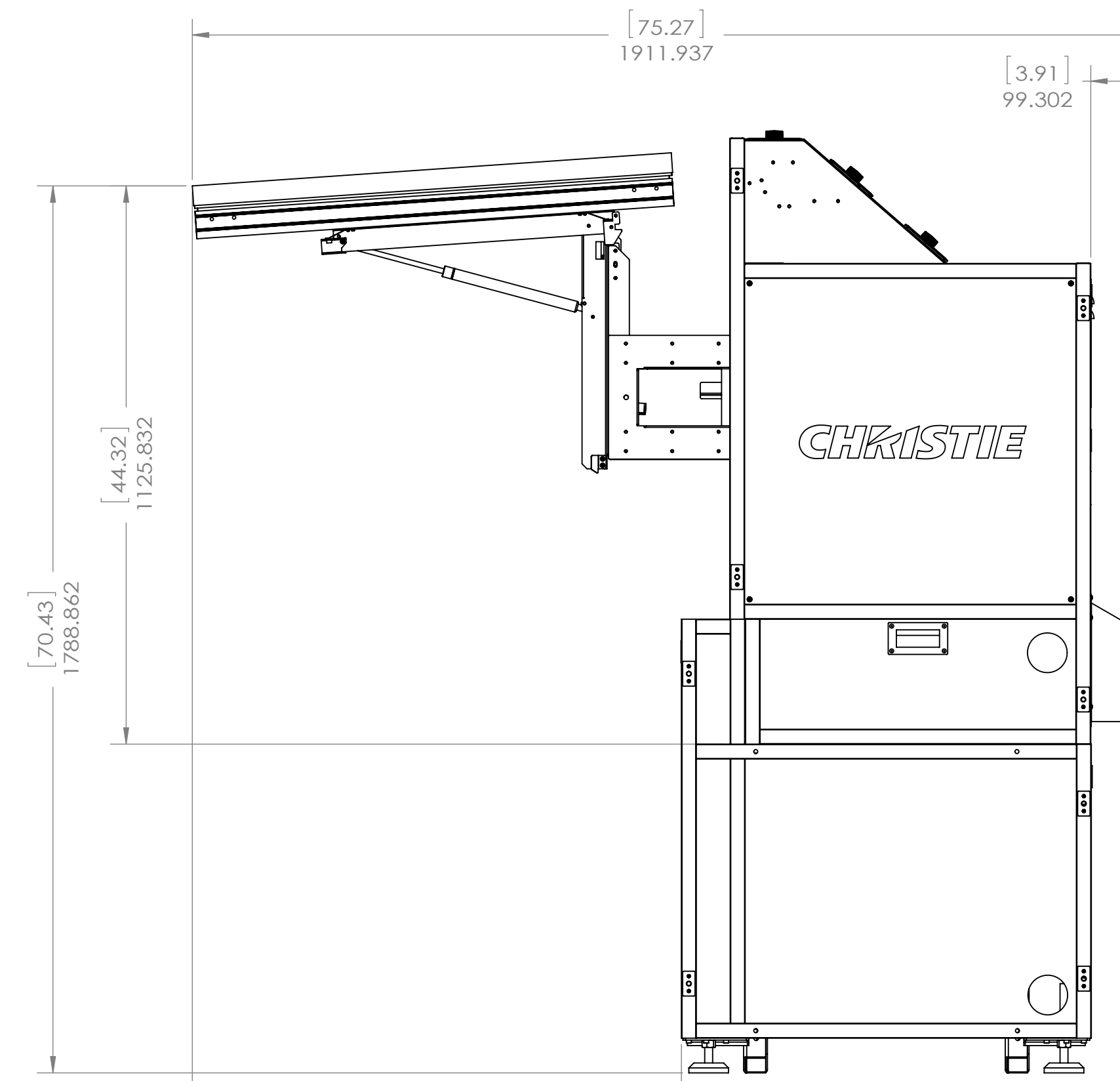
SIDE VIEW
