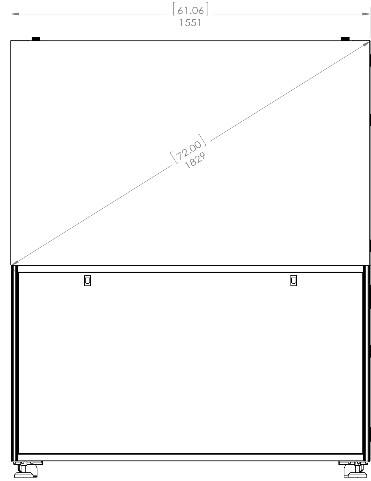
FRONT VIEW
