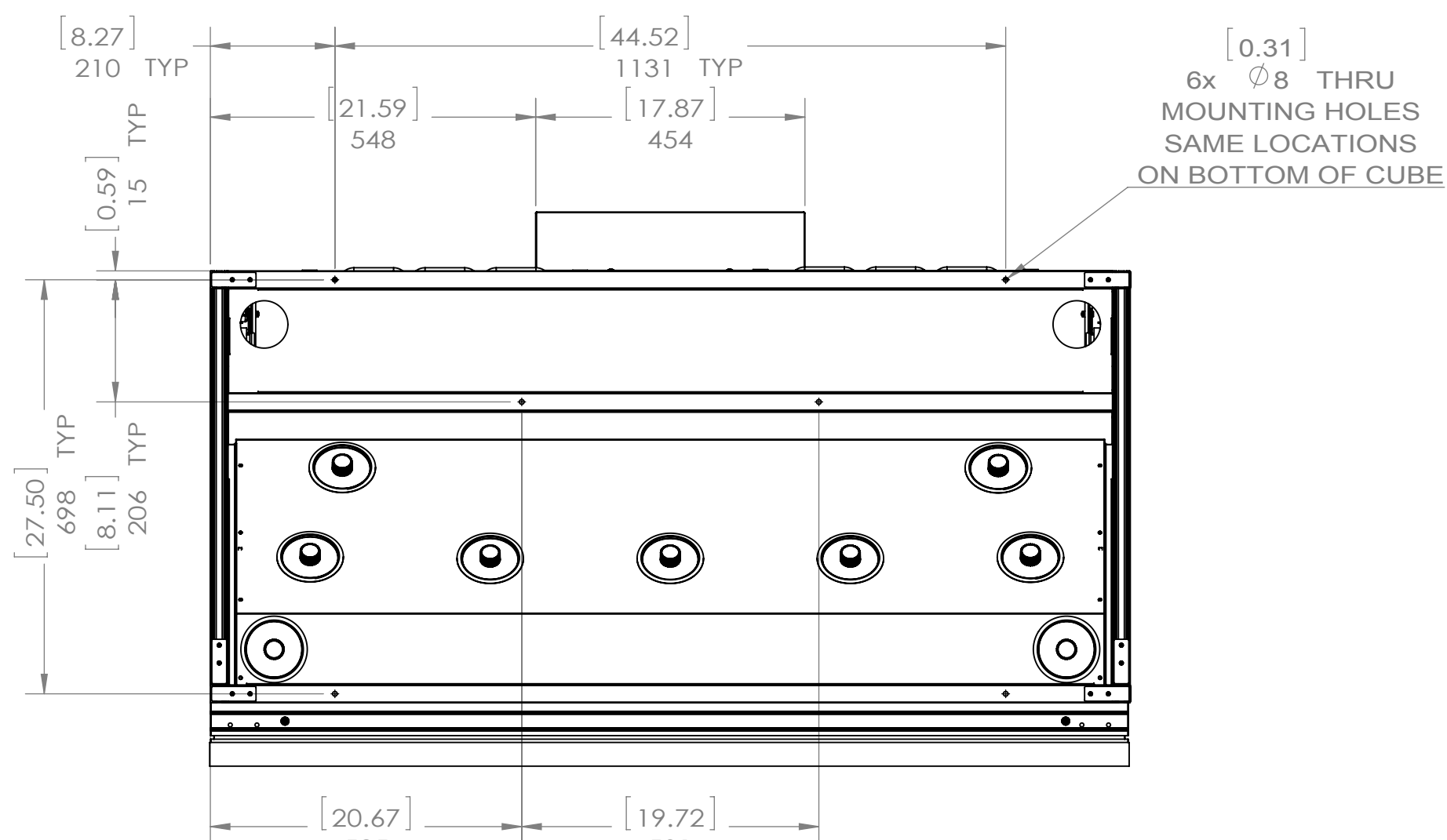
TOP VIEW
