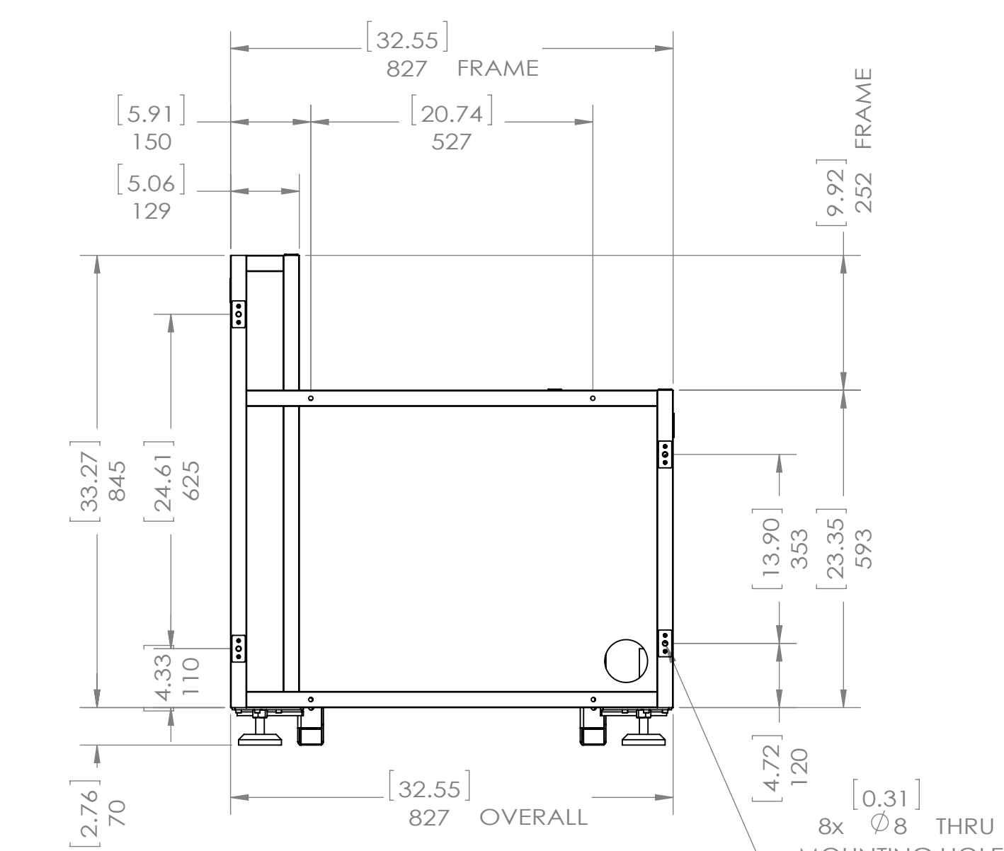
SIDE VIEW
