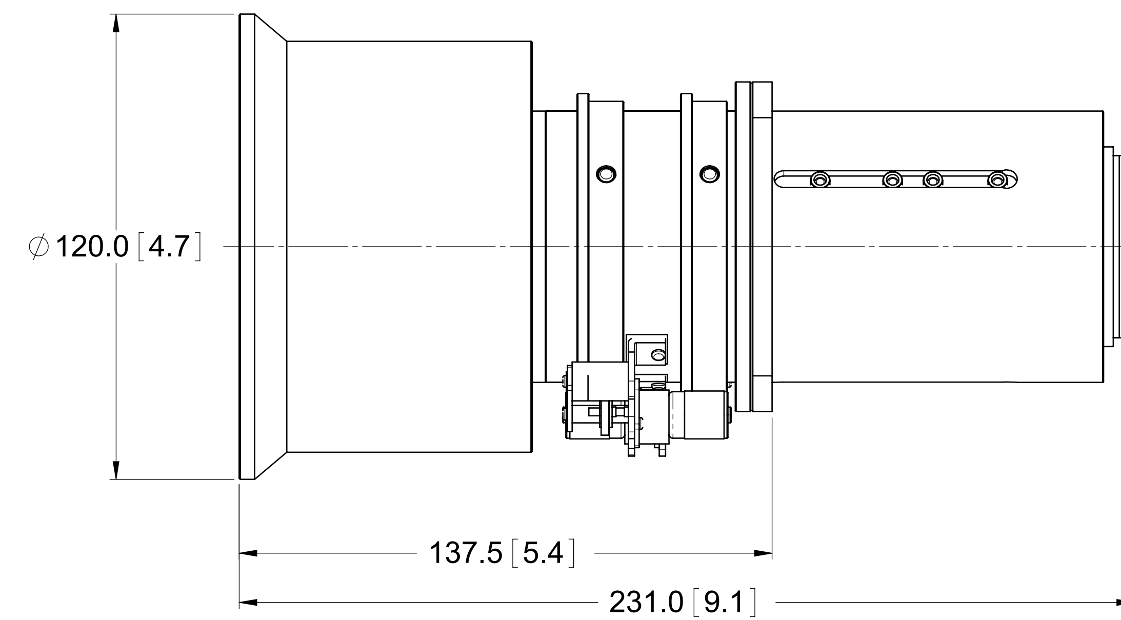
133-103105-XX 2.0-4.0:1 ZOOM
