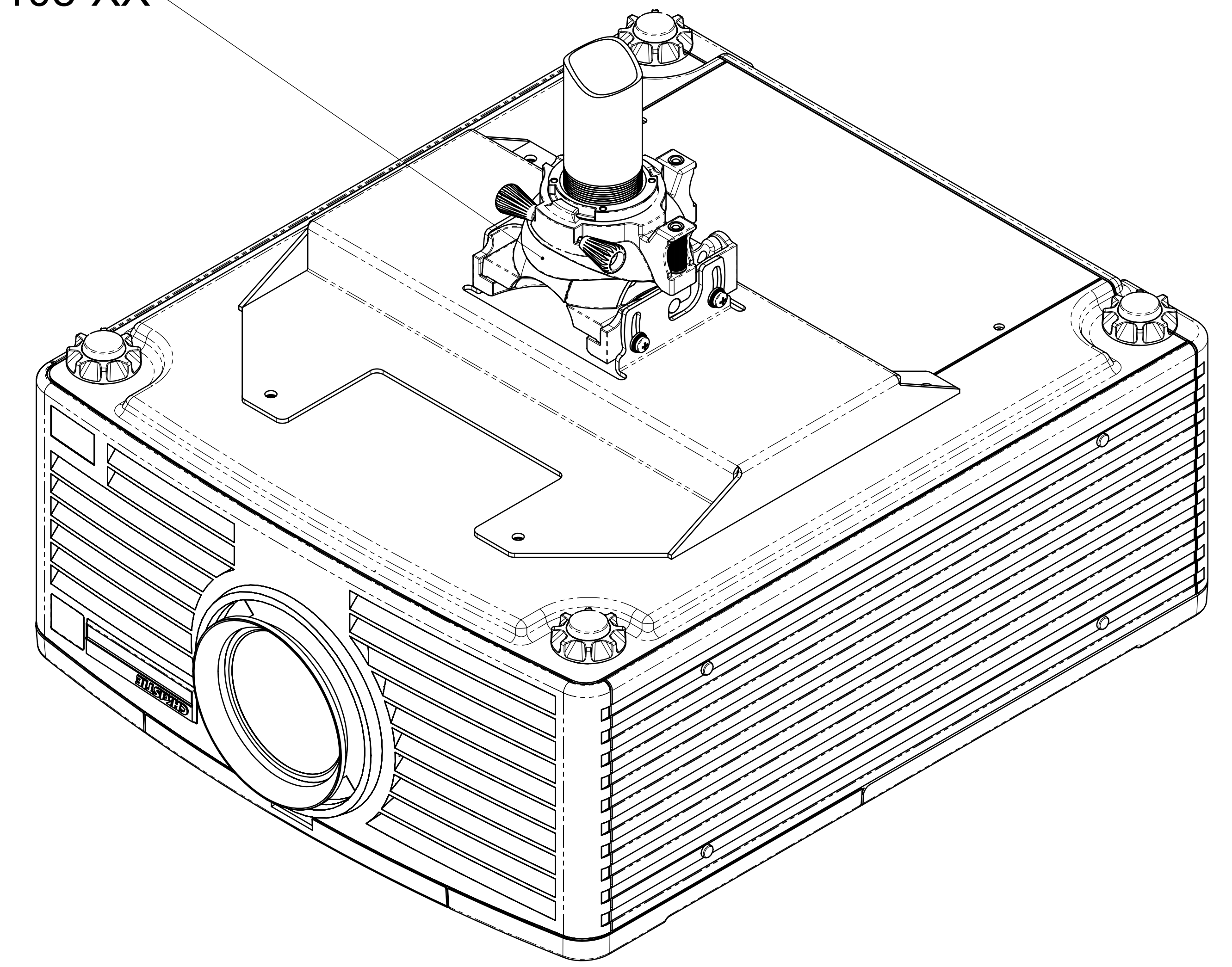
ISOMETRIC VIEW
