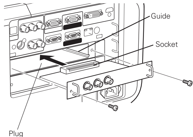
Figure shows Dual SDI Board
