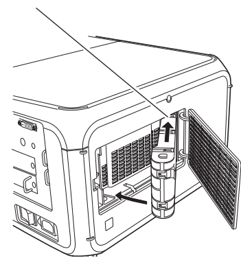
Filter cartridge
